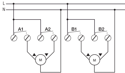
2 canales de Persiana / 2 Shutter/Blind channels
