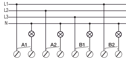
4 canales On/Off en Trifásica / 4 On/Off channels with three-phase voltage
